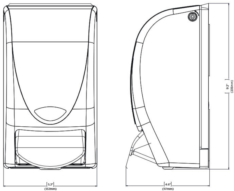
1 LITER MANUAL DISPENSER
