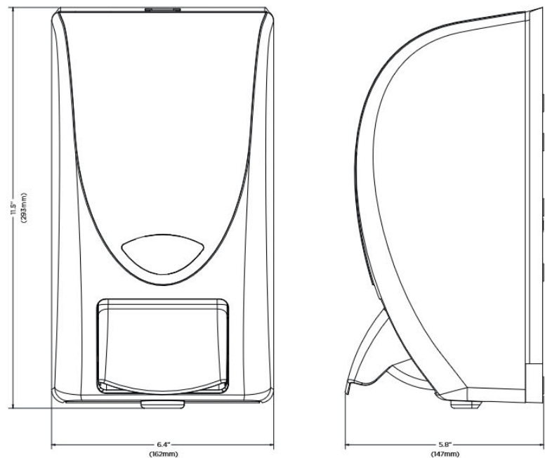
2 LITER MANUAL FOAM DISPENSER
