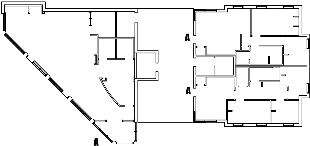
B/C FIRST FLOOR PLAN
